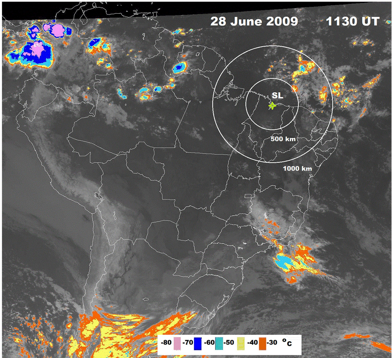
Figure 4. Image from GOES satellite at 11:30 UT on 28 June 2009 showing the presence of convective zones near São Luis.
