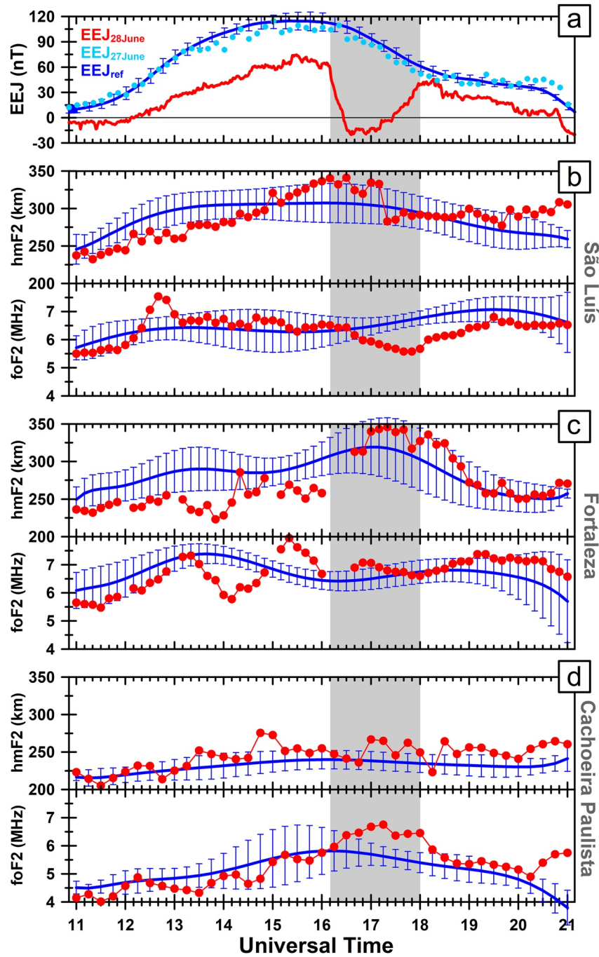
Figure 2. From top to bottom are shown: the equatorial electrojet (EEJ) strength over Brazil (panel a) during 27 (cyan dots) and 28 June 2009 (red curve) with the respective quiet-time reference (panel a, blue curve); F_2 layer peak height -hmF_2 and the F_2 layer critical frequency -foF_2 (red dots) over SL (panel b), FZ (panel c) and CP (panel d). The average quiet days hmF_{2ref} and foF_{2ref} and their respective standard deviations are represented by the blue curves. The solid blue curves, indicated in panels b–d represent the smoothing made in average data, hmF_2 and foF_2 using polynomial interpolation. The plots are in function of universal time (UT = LT + 3 h).
